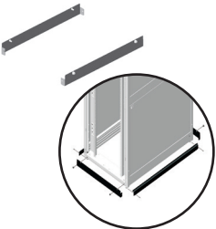
Seal Kit Installation
